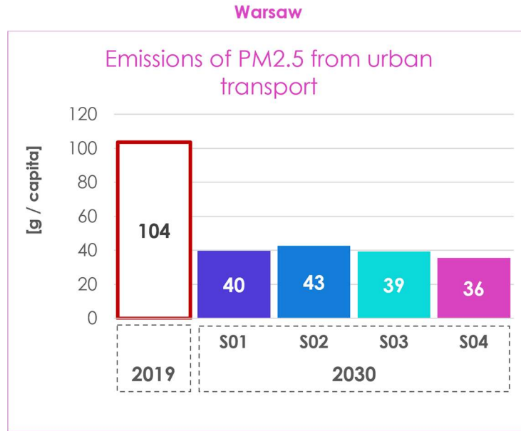
Figure 12: Emissions of PM2.5 in Warsaw
