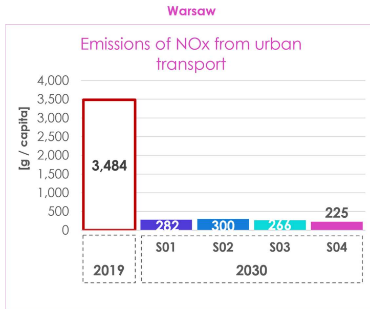
Figure 13: Emissions from NOx in Warsaw
